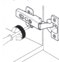
Height adjustment
